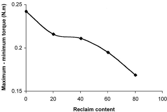
FIGURE 2 Variation of (maximum–minimum) torque with reclaim loading.
