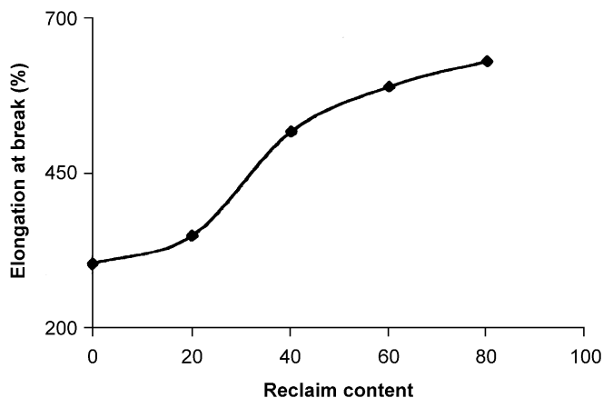
FIGURE 7 Variation of the elongation at break with reclaim loading.
