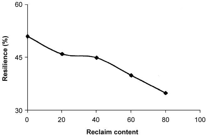
FIGURE 9 Variation of resilience with reclaim loading.
