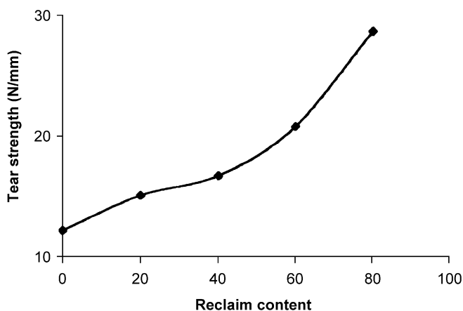
FIGURE 8 Variation of the tear strength with reclaim loading.
