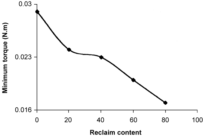
FIGURE 1 Variation of minimum torque with reclaim loading.
