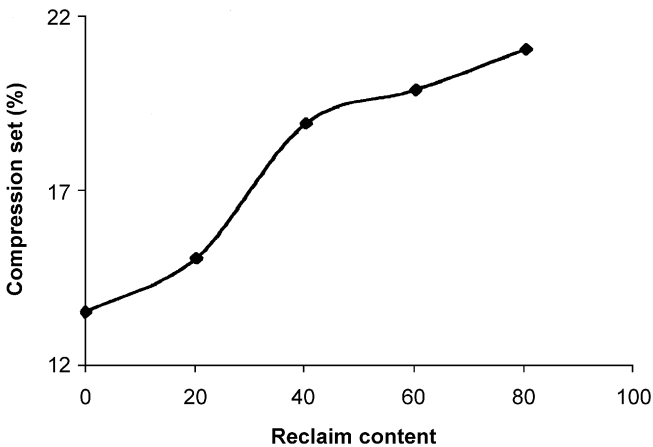
FIGURE 10 Variation of compression set with reclaim loading.
