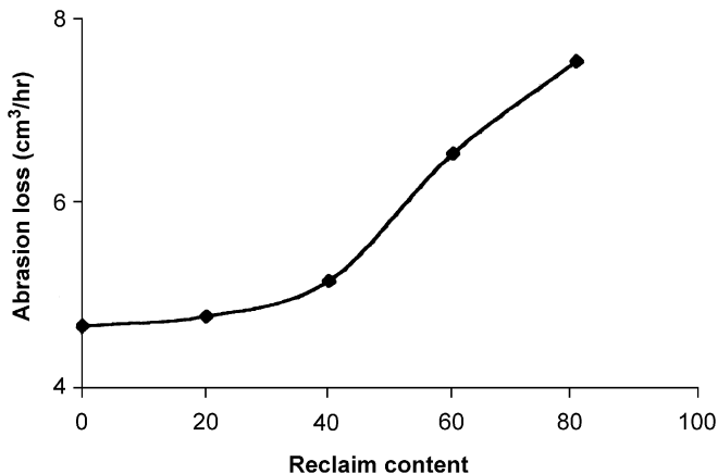
FIGURE 11 Variation of the abrasion loss with reclaim loading.
