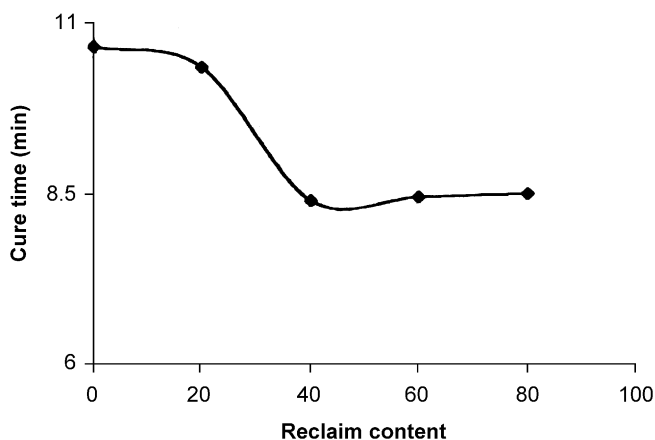
FIGURE 4 Variation of the cure time with reclaim loading.
